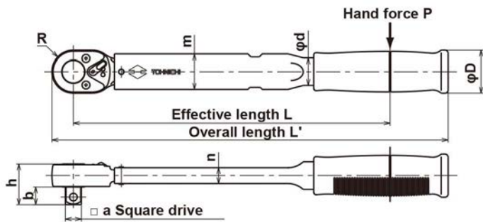
BQSP10N~BQSP300N
